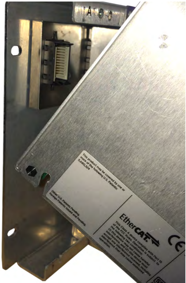
Figure 2 Notch for Module Alignment
