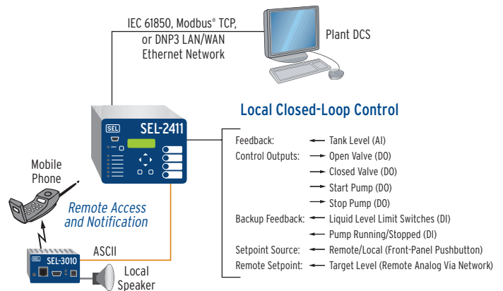
Level control example.
