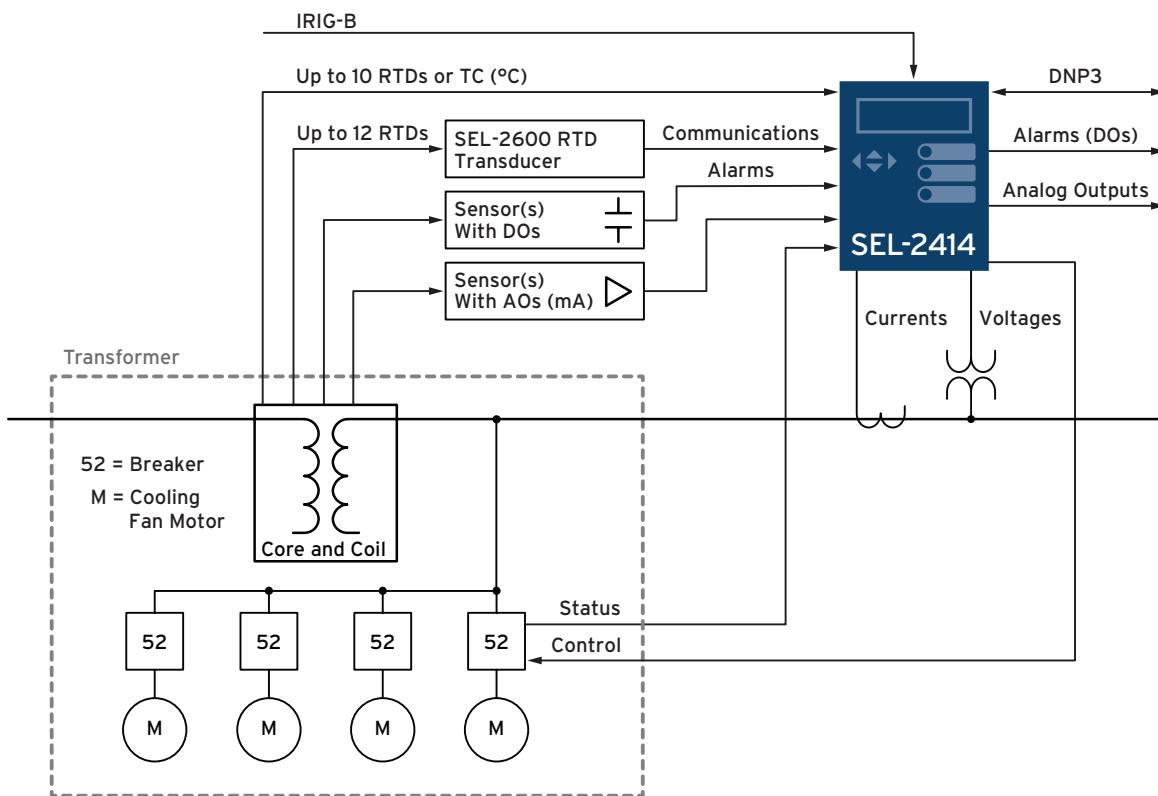
Transformer monitor system example.
