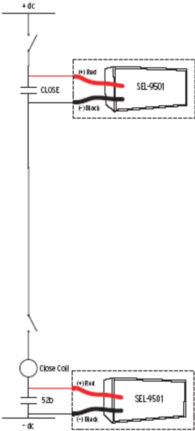
Typical SEL-9501 Contact Arc Suppressor Applications (160 Vdc Maximum)
