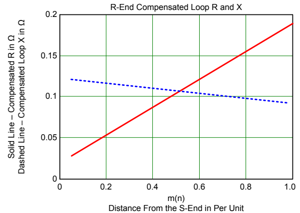
Fig. 8 R-end compensated loop R and X in \Omega for a single-phase-to-sheath fault on a single-point bonded cable
