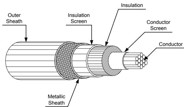
Fig. 1 XLPE cable construction
