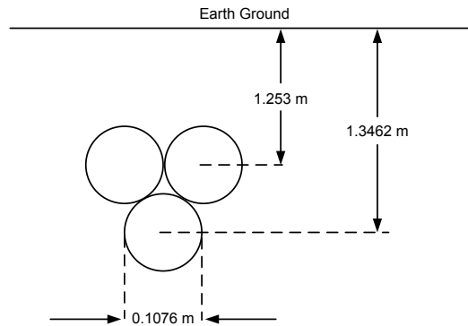
Fig. 18 Cable trefoil configuration
