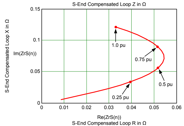
Fig. 12 Nonlinear behavior of compensated loop impedance in solid-bonded cables
