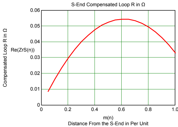
Fig. 14 Compensated loop resistance at Terminal S
