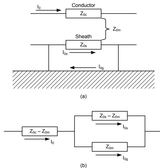
Fig. 19 Zero-sequence return currents and equivalent circuit
