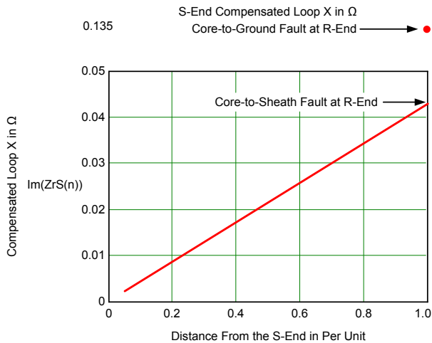
Fig. 6 S-end compensated loop reactance in \Omega for a single-phase-to-sheath fault on a single-point bonded cable
