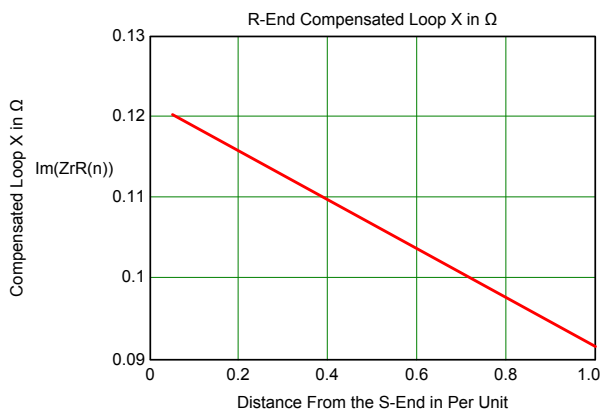
Fig. 7 R-end compensated loop reactance in \Omega for a single-phase-to-sheath fault on a single-point bonded cable
