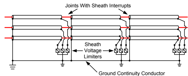
Fig. 2 Single-point bonding
