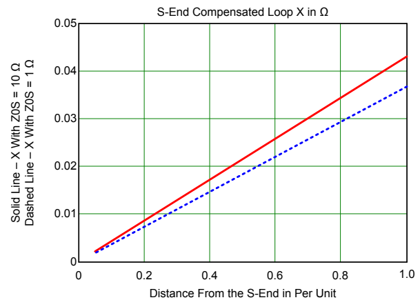
Fig. 9 Variation of the compensated loop reactance at Terminal S caused by a change of the zero-sequence source impedance magnitude
