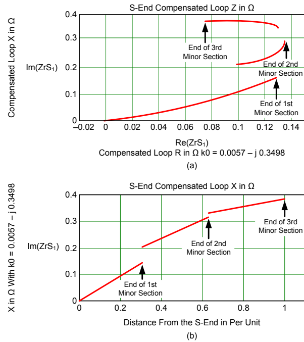
Fig. 15 Compensated loop impedance (a) and reactance (b) for cross bonded cables
