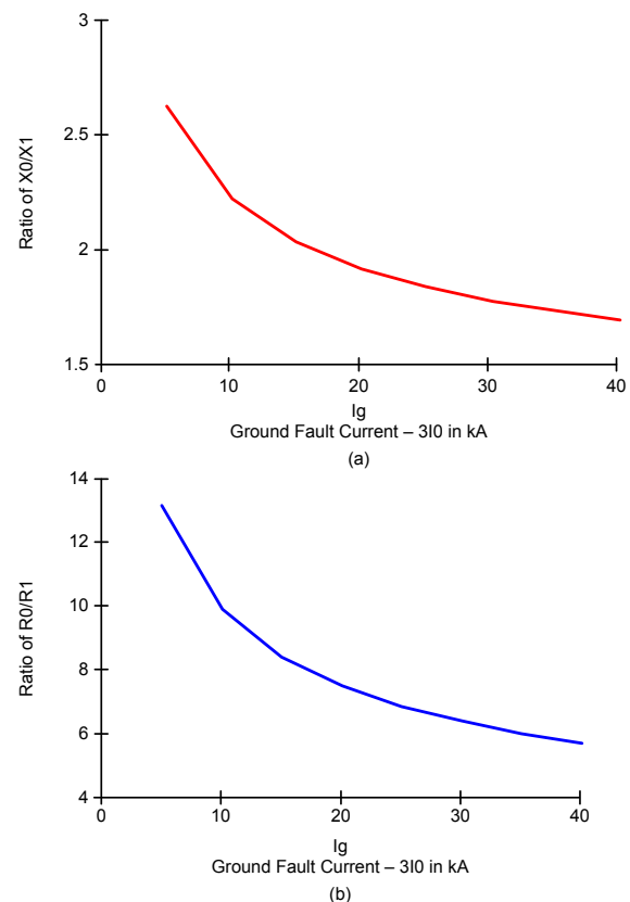
Fig. 4 Variation of zero-sequence resistance and reactance in a 230 kV pipe-type cable as a function of ground fault current
