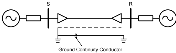
Fig. 5 Single-point bonded cable at Terminal S
