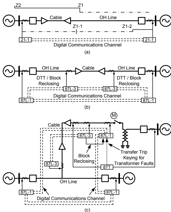
Fig. 17 Mixed overhead and underground circuits
