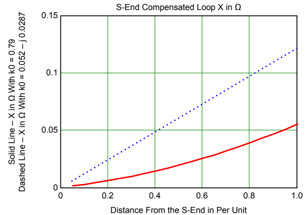
Fig. 13 Compensated loop reactance for different values of zero-sequence current compensation factors
