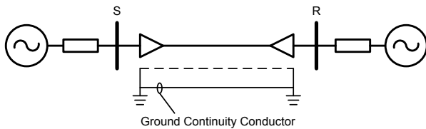
Fig. 10 Solid-bonded cable with sheaths grounded at both ends of the cable
