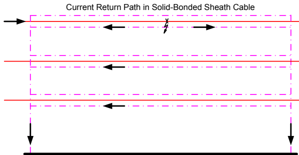
Fig. 11 Paths for ground current return for a core-to-sheath fault in single-conductor solid-bonded cables
