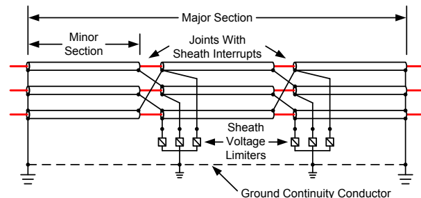
Fig. 3 Cross bonding
