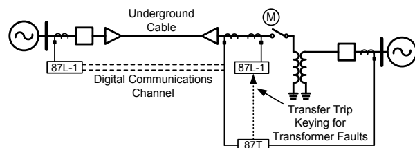
Fig. 16 EHV cable terminated into a transformer
