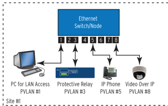
Fig. 9. Port-Based VLANs
