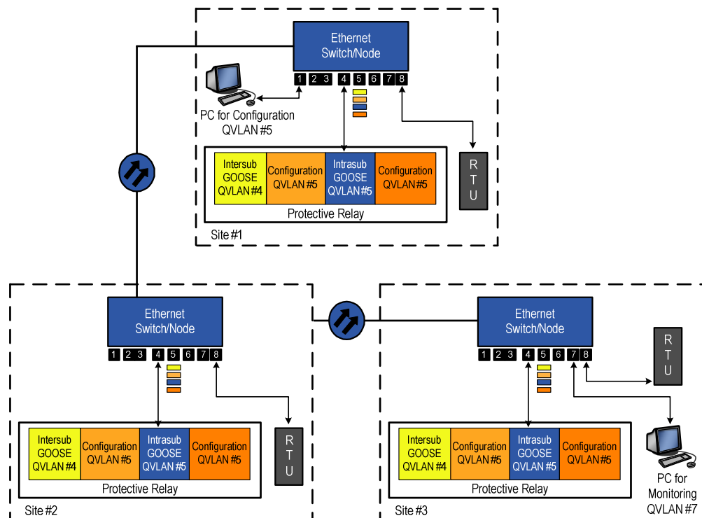
Fig. 10. Substation Implementation
