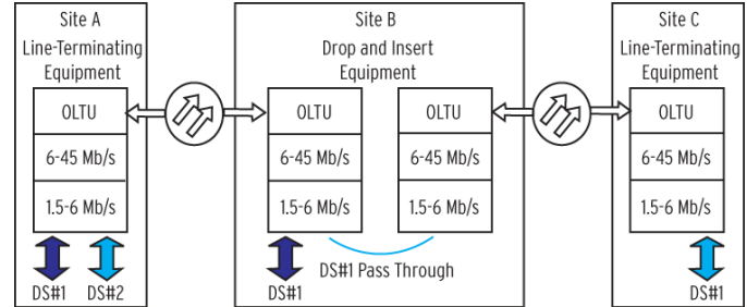
Fig. 2. PDH Network
