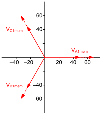
Fig. 18 BCG fault relay vectors; dashed lines represent expanded memory voltage vectors, and solid lines represent steady state.
