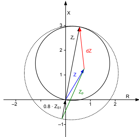
Fig. 19 Phase-to-ground fault dynamic mho characteristic (steady state).
