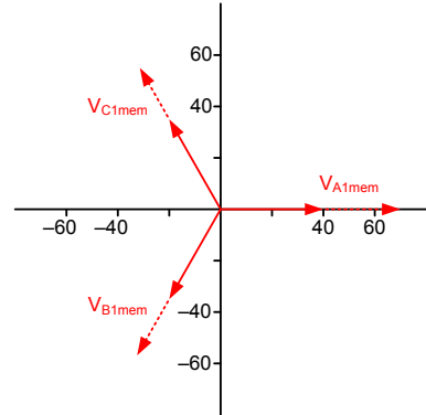
Fig. 11 Three-phase fault relay vectors; dashed lines represent expanded memory voltage vectors, and solid lines represent steady state.
