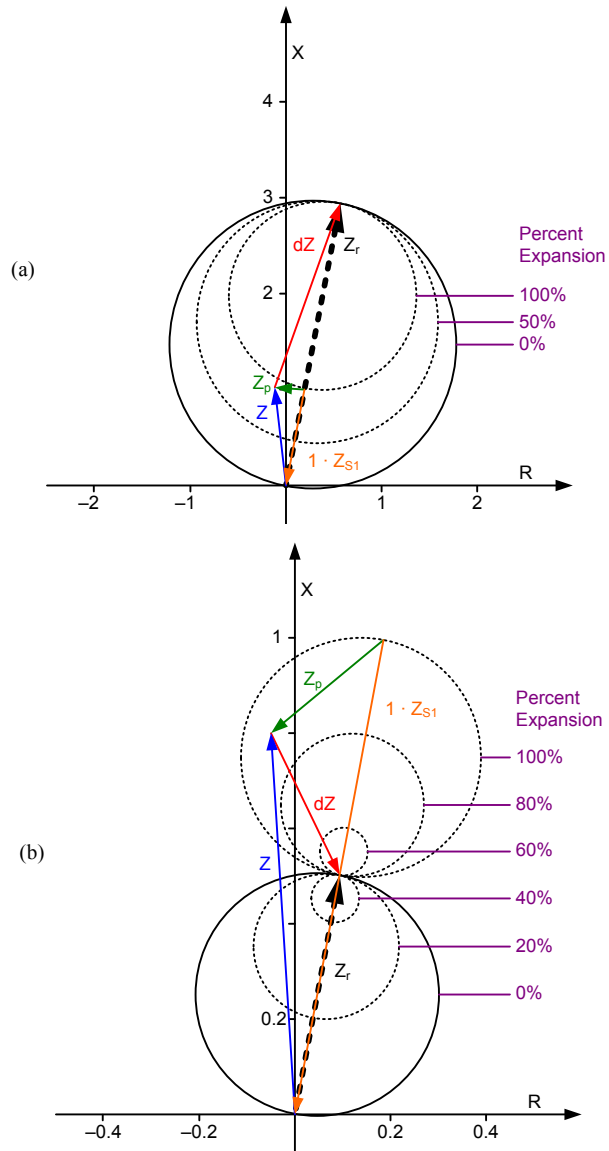
Fig. 32 Impedance diagram for Relay R2 in response to a reverse three-phase fault on the opposite side of the series capacitor: (a) Case I: |Z_r| > |X_C| , (b) Case II: |Z_r| < |X_C| .
