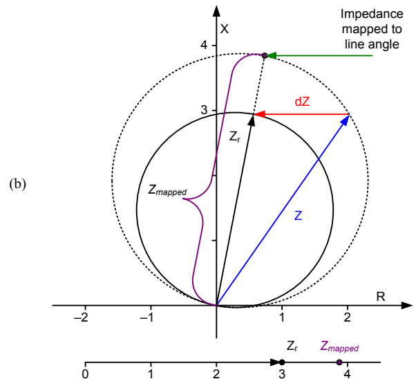
Fig. 5 Mapping a measured impedance to the line angle and corresponding number line for (a) A fault within reach point, (b) An external fault.
