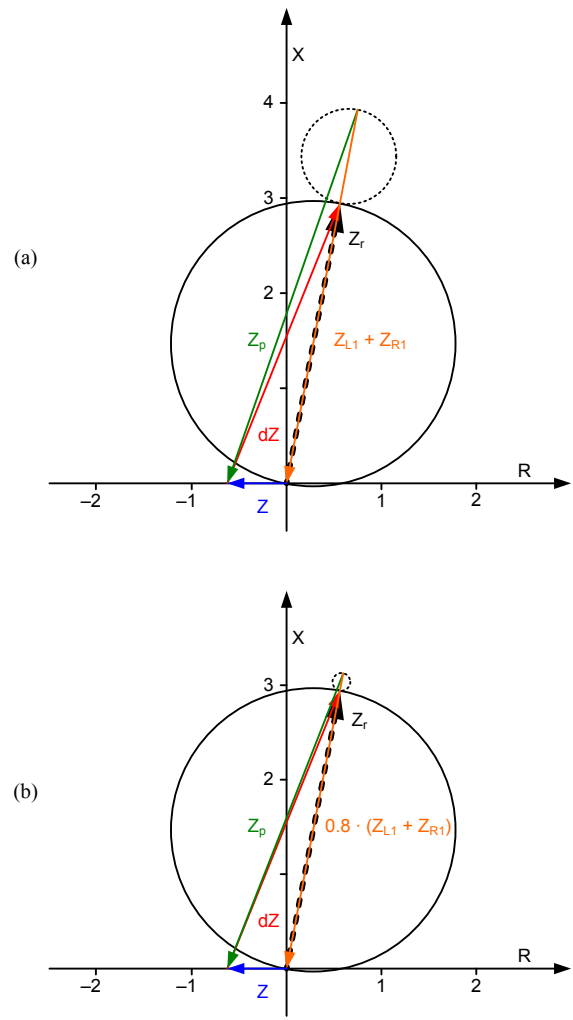
Fig. 22 Close-in reverse phase-to-ground fault dynamic mho characteristic with arc resistance added: (a) Maximum expansion, (b) Steady state. Note that the dynamic mho (dashed circle) determines operation. The self-polarized mho (solid circle) is shown as a reference.
