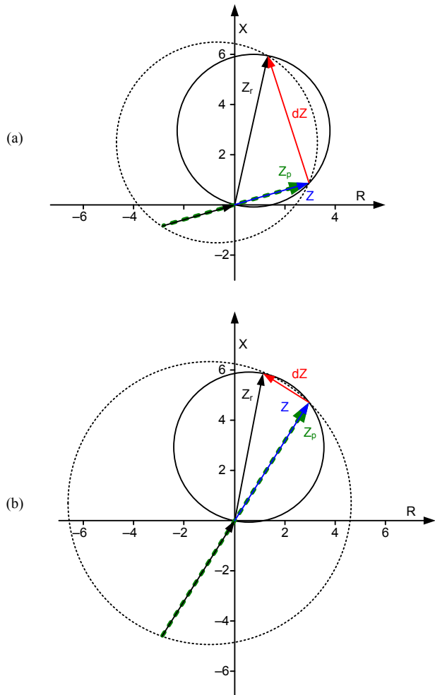
Fig. 26 Common test values for an AG fault; the dynamic mho does not interfere with testing when the angle of V_A and V_{Imem} are equal: (a) Test 1, (b) Test 2.
