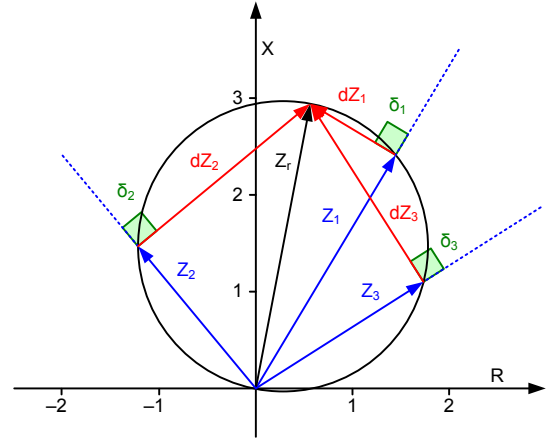
Fig. 3 Right-angle property of a circle.
