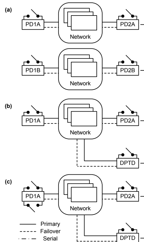
Fig. 4. Complete Dual-Primary Signaling Systems (a) Application of DPTD (b) and Dual-Input Contacts (c).
