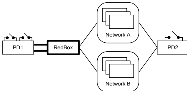
Fig. 8. Primary and Failover Cables, Singly Attached Node.
