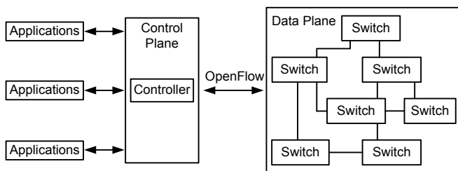
Fig. 10. SDN Architecture Overview.
