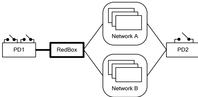
Fig. 7. Single Cable, Singly Attached Node.
