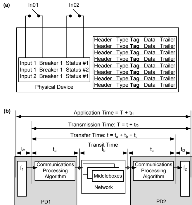
Fig. 3. IED Contact Input Information Mapped as Payload Data in GOOSE Messages (a) and Application, Transmission, Transfer, and Transit Time Based on IEC 61850-5 (b).
