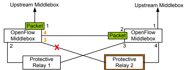
Fig. 11. OpenFlow Group Port Failover.
