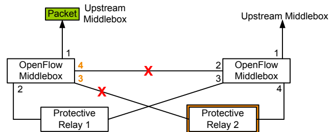
Fig. 12. OpenFlow Outputs Packet to Original Ingressing Port.
