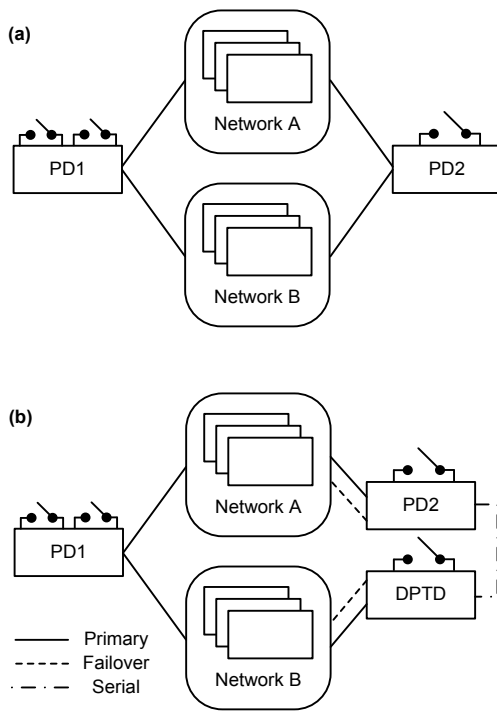
Fig. 6. Redundant Information Via Dual-Primary Contact Inputs (a) and Redundant Application Via a DPTD (b).
