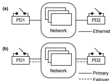
Fig. 2. System Exchanging Protection Signals in Ethernet Packets Through a Network (a) and Duplicate Ethernet Cable Serving as Hot Standby (b).
