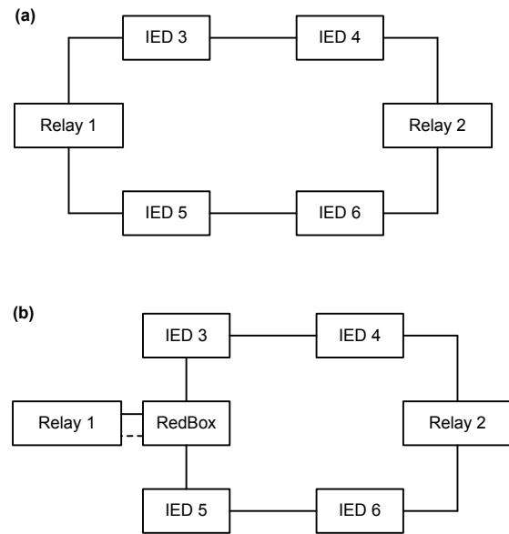
Fig. 9. Redundant Packets Within Single HSR Network Ring (a) and Non- HSR-Enabled Relay Connected Via RedBox (b).
