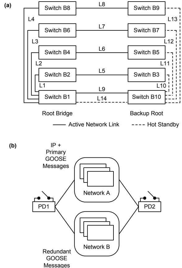
Fig. 5. Resilient Single Primary Ladder Network Topology (a) and Dual-Primary Signaling Via Two Systems Segregated by QVLANS (b).
