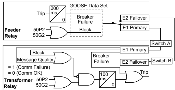
Fig. 1. Use of GOOSE Message Quality Status in IED Logic.
